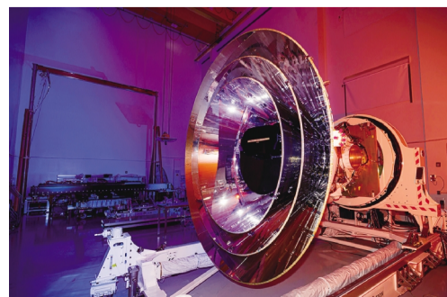
SPHEREX' CO12NASA
